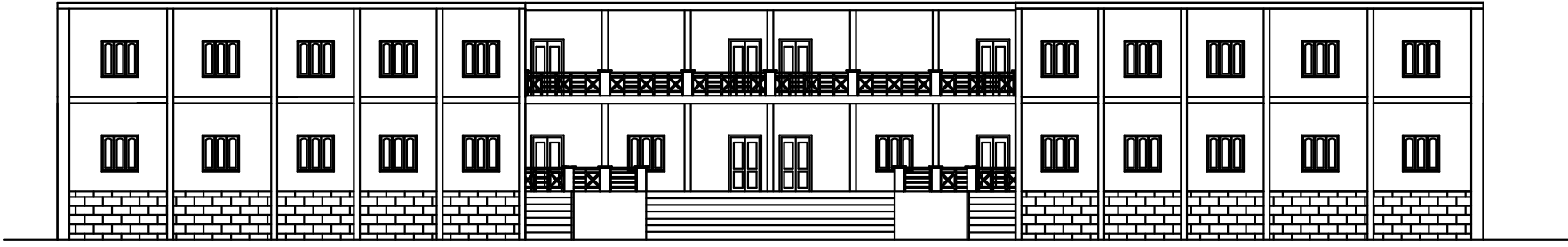
FRONT ELEVATION
